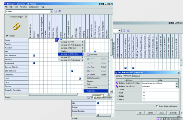
Matrix View Supports Fast & Easy Linking
